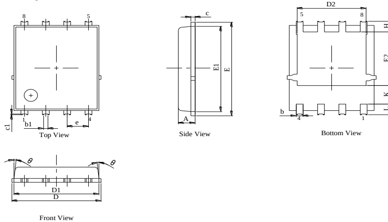
Package Outline
